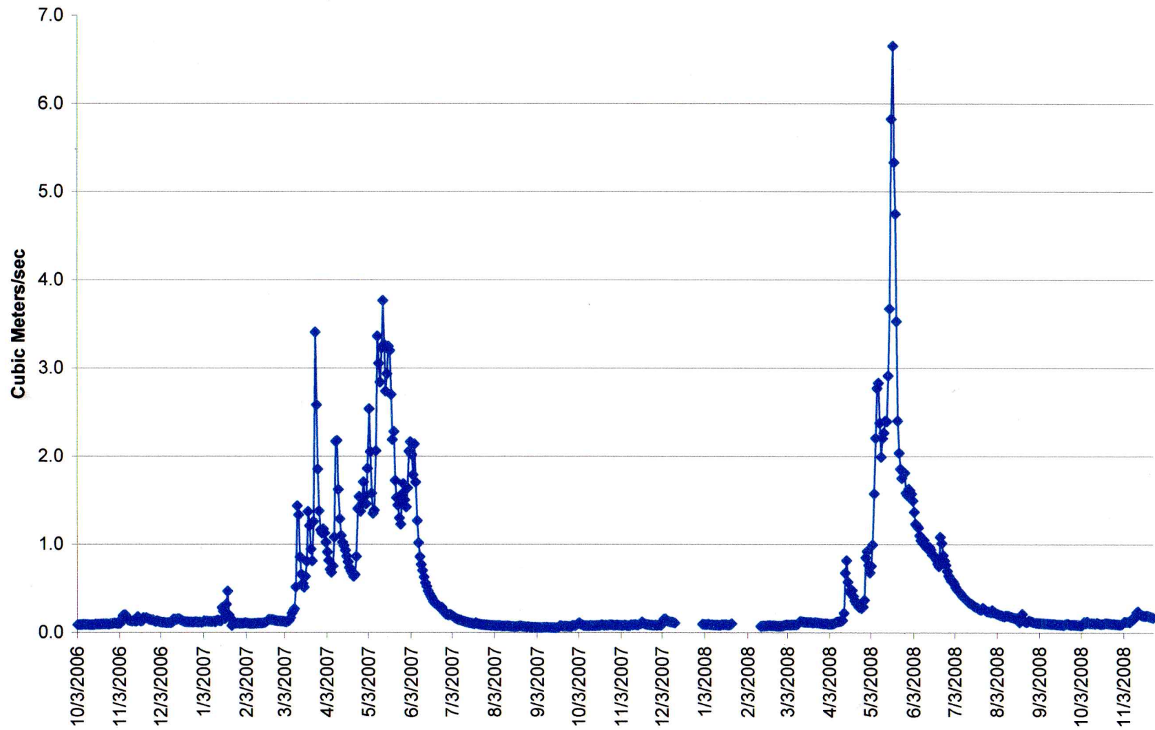
Winlaw Daily Mean Flow 2006-8
